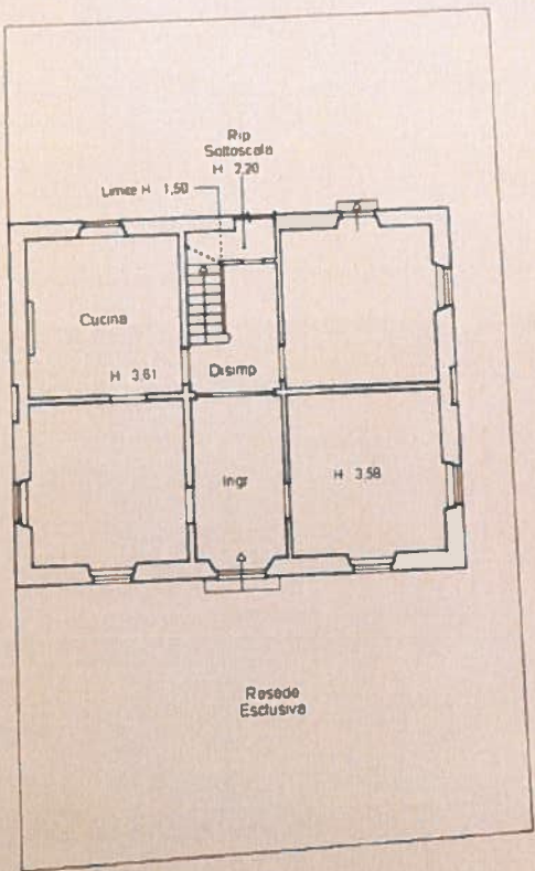
Piano Terra
