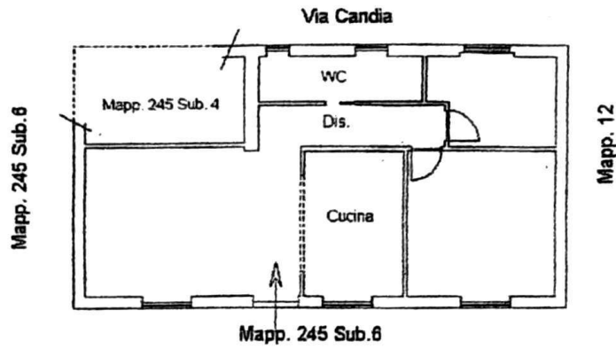
Pianta Piano Terra h= ml 2.80
