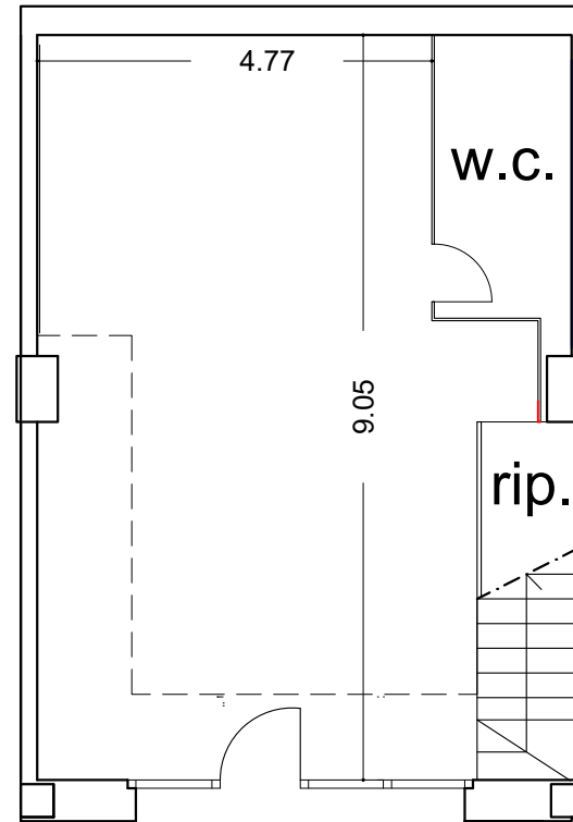
▲ piano terra
