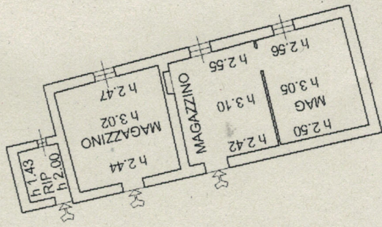
PIANO TERRENO
