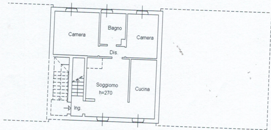
Pianta Piano 2
