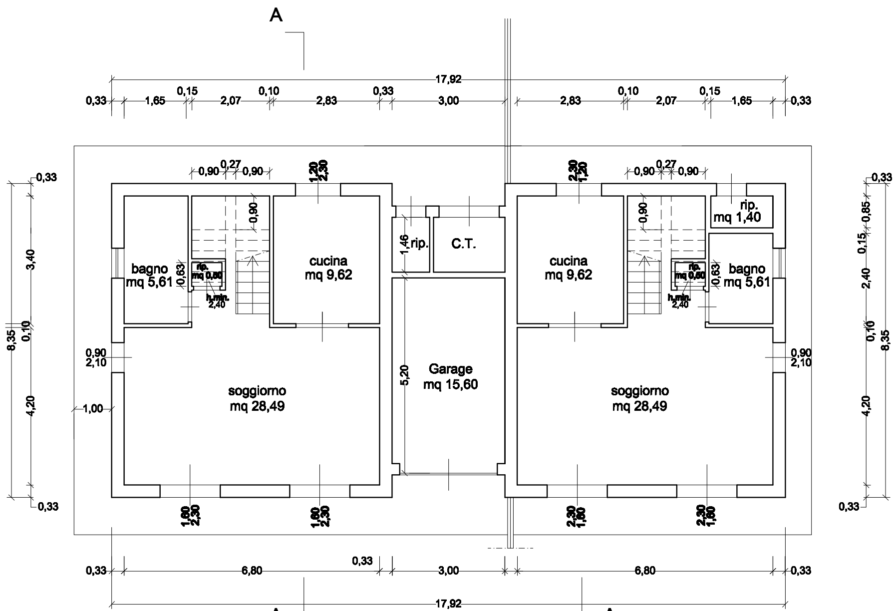
PIANO TERRA
