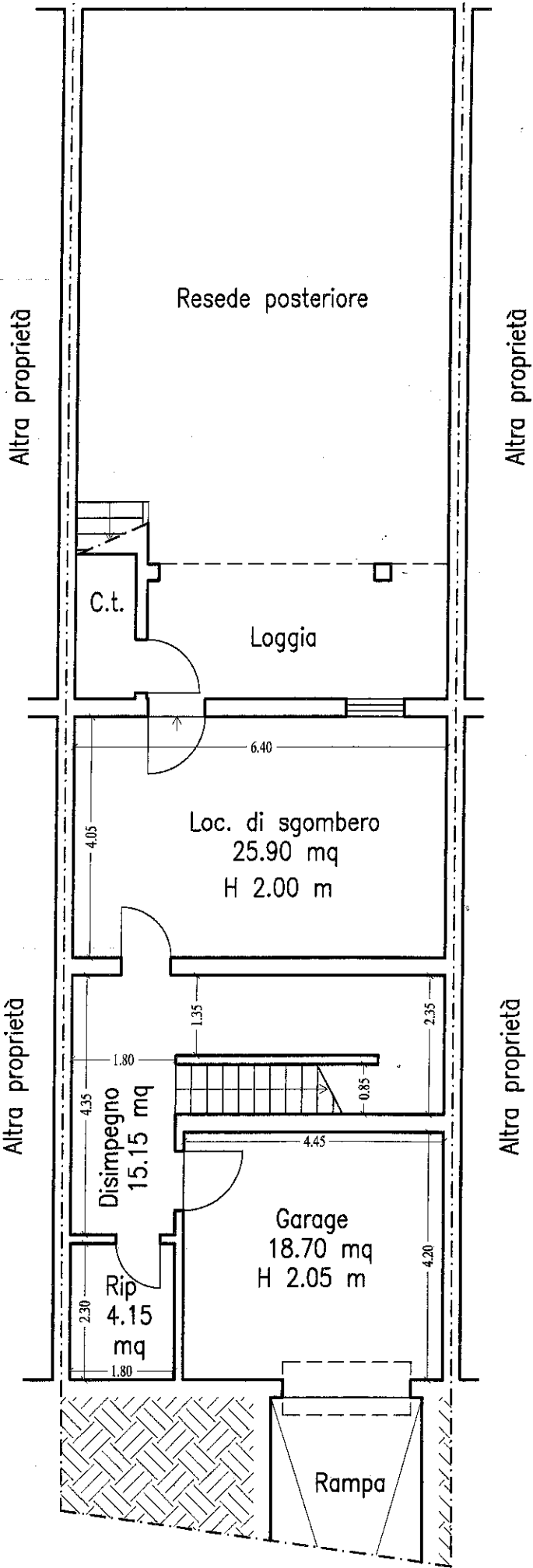
PIANO SEMINTERRATO
