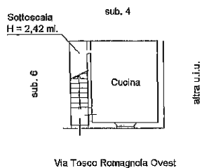
Pianta Piano Terra H = 2,65 ml. part. 59 sub. 7
