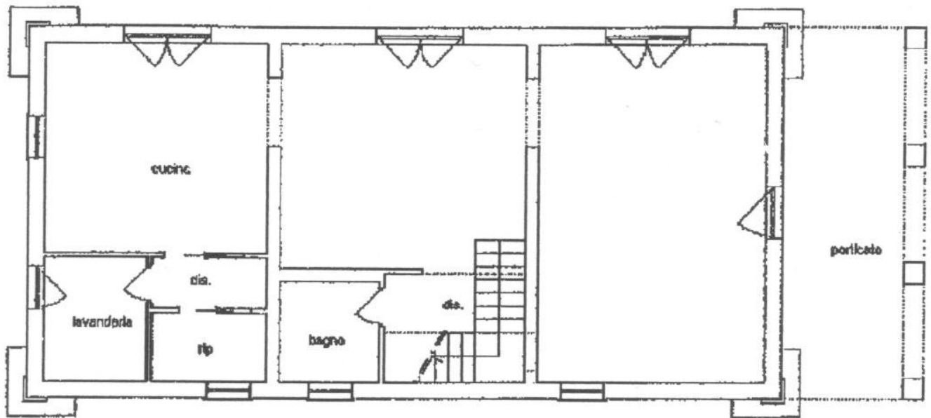
PIANO TERRA h 3.00
