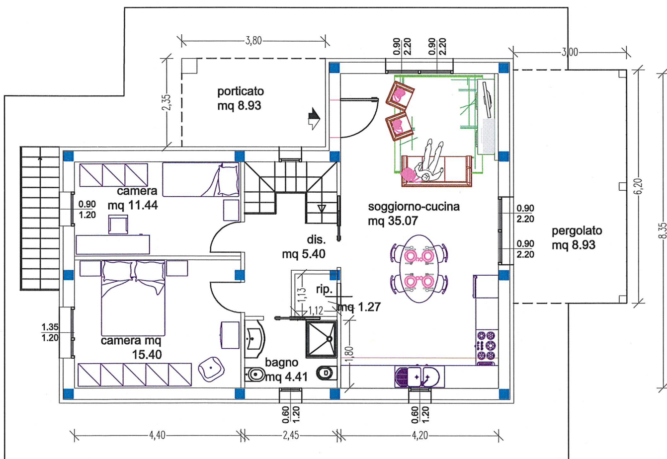
PIANO TERRA
